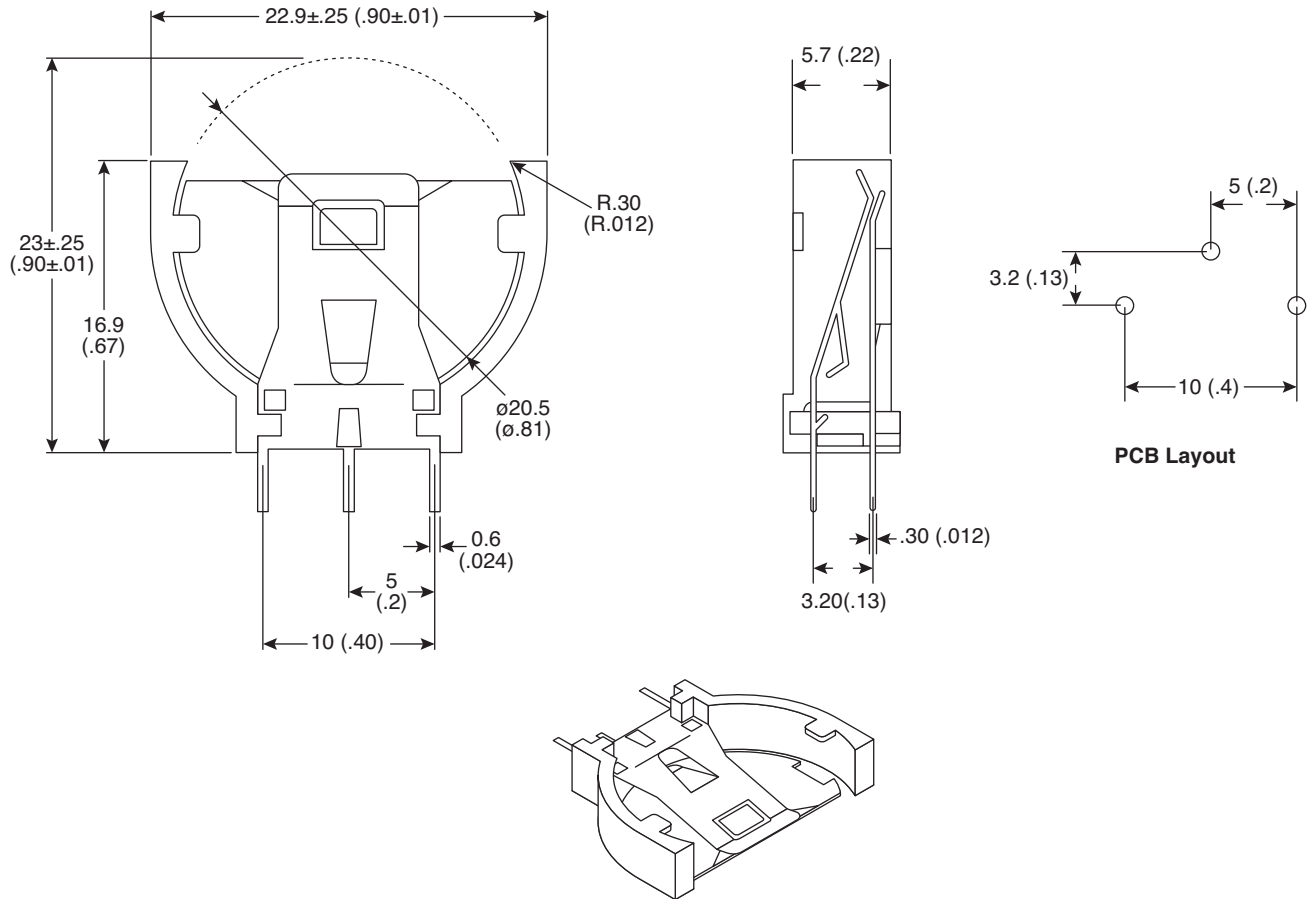
Dimensions: mm (in.)
